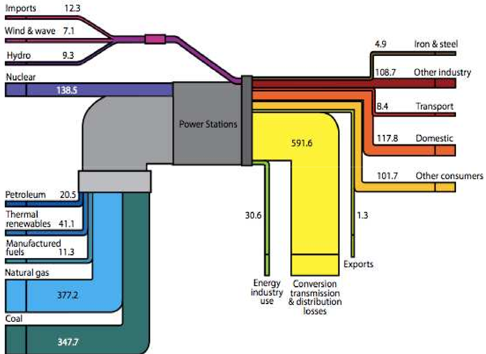
Fig. 8.1 UK electricity flow chart
