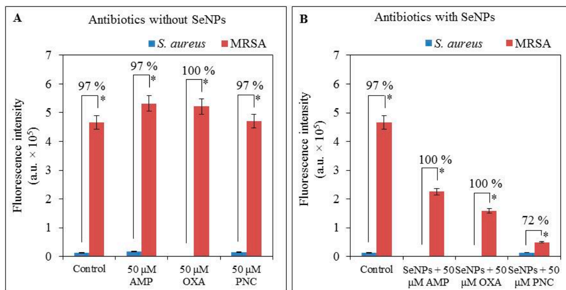
Figure 3. Monitoring of mecA gene expression in bacterial strains S. aureus and MRSA after 24 h of growth with (A) 50 \mu\text{M} ATBs concentration and with (B) 100 \mu\text{M} concentration of SeNPs with 50 \mu\text{M} ATBs concentration in complexes using PCR and subsequent gel electrophoresis. Controls are bacterial strains ( S. aureus and MRSA) without application of antibacterial component. All data represent mean \pm S.D. NS, not significant, * p < 0.05 .
